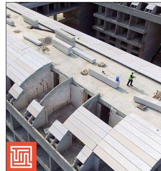
YTONG ÇATI PLAĞI Ytong Roof Plate
