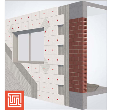
MULTİPOR M. SİSTEMİ Multipor Insulation System
